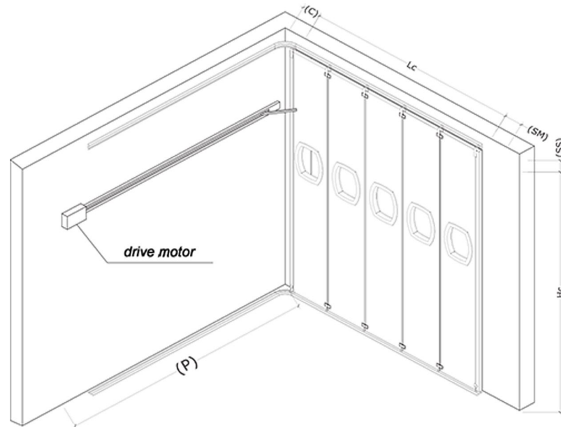
Example of Typical Installation
